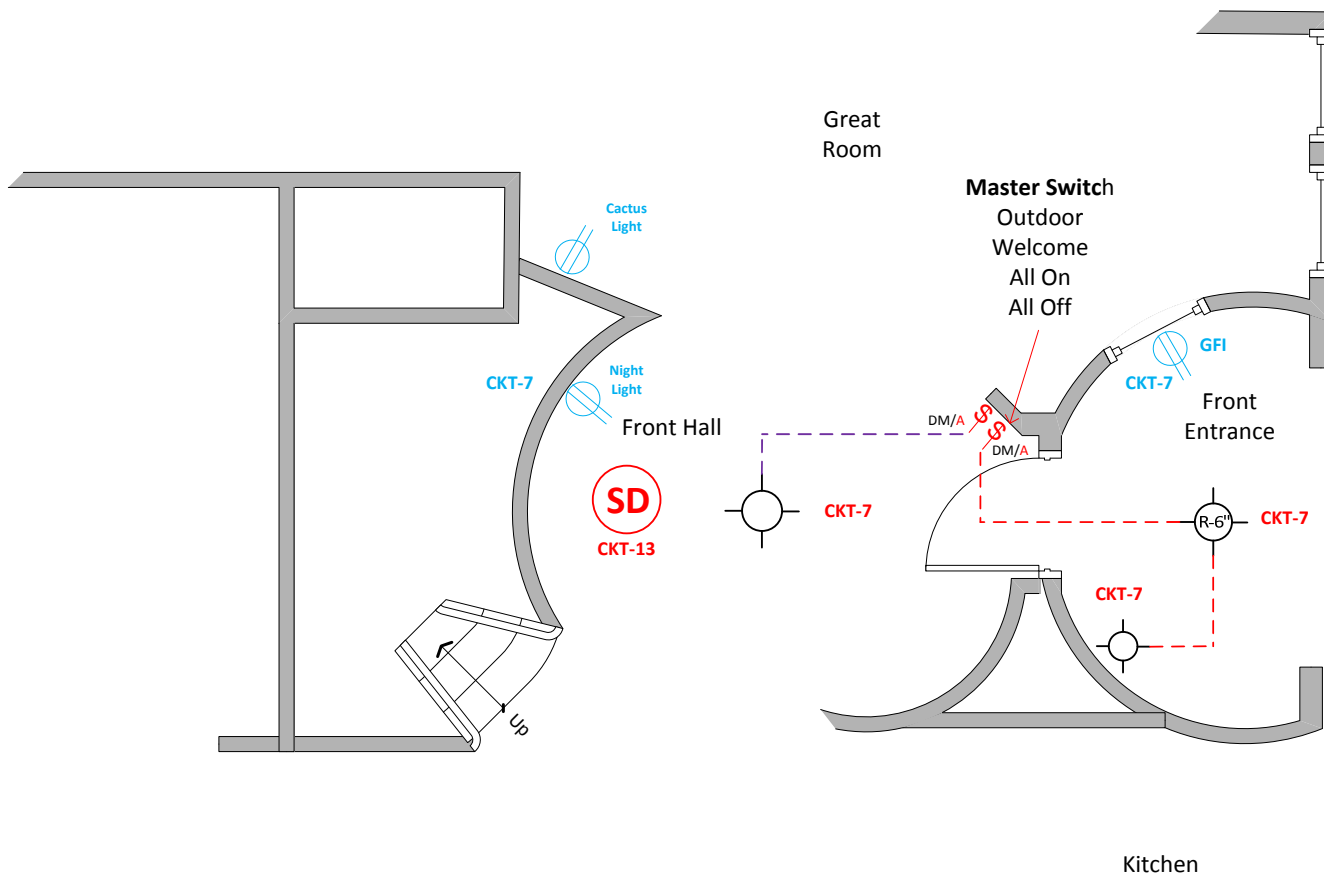
FRONT ENTRY LIGHTING / SWITCH LAYOUT RECEPTACLES
