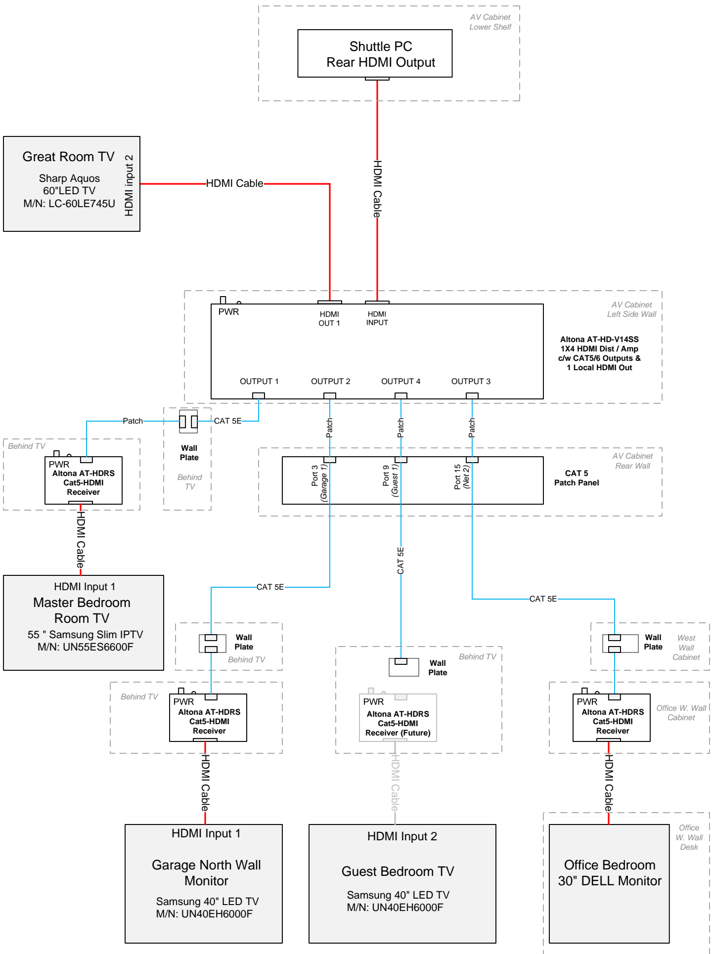
COMPUTER DISPLAY DISTRIBUTION
